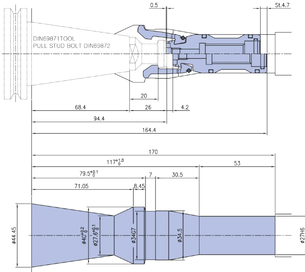
Spindle Detail
